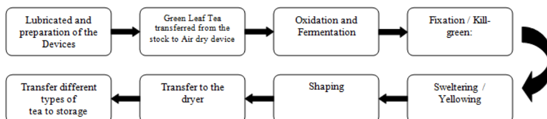
Figure 1. The production process in Soofi Tea Factory.
